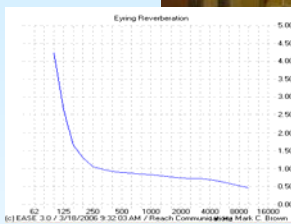
Gym RT60 Profile, Example EASE Acoustics Project 2006
